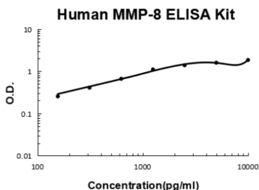
Human MMP-8 PicoKine ELISA Kit standard curve
